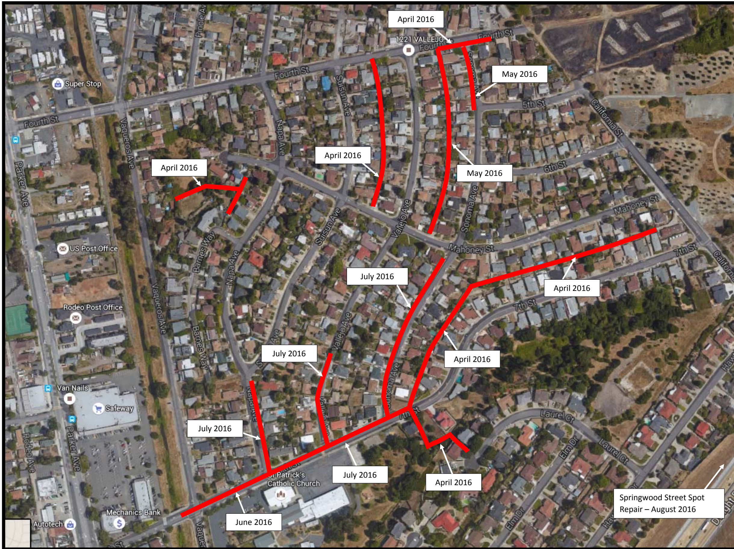
FIGURE 1 Preliminary Construction Schedule Sewer Year 2A Project
